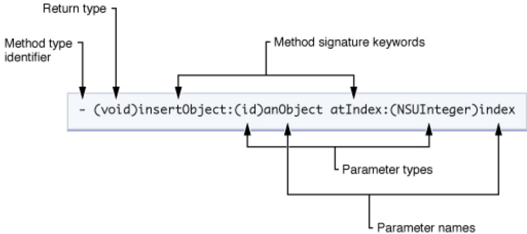
Figure 2 Method declaration syntax
