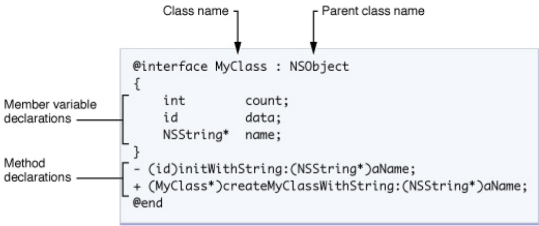
Figure 1 A class declaration
